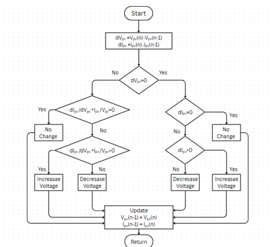
Fig.2: Incremental Conductance (INC) with Fuzzy Logic Flow chart.
