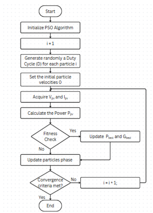
Fig.4: Particle Swarm Optimization (PSO)-Based MPPT Flowchart.
