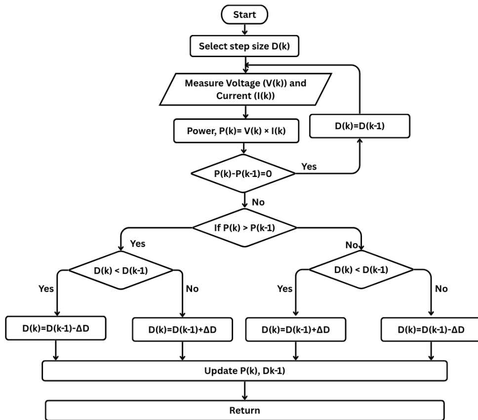
Fig.1: Perturb and Observe (P&O) with Adaptive Step Size Flow chart.
