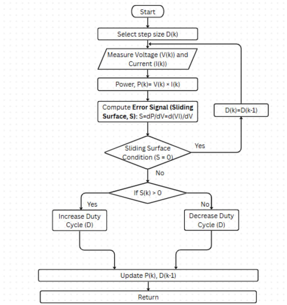
Fig.6: Sliding Mode Control (SMC)-Based MPPT Flowchart.
