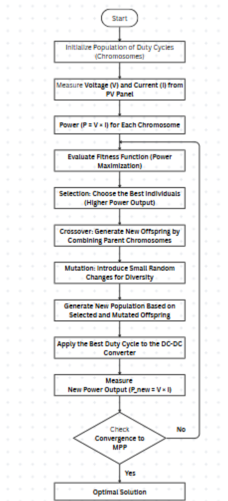
Fig.5: Genetic Algorithm (GA)-Based MPPT Flowchart.
